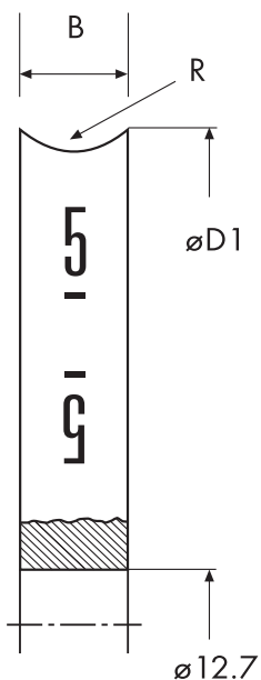
Molette concave
