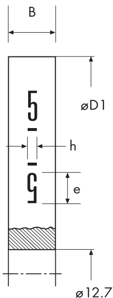
Molette plane
